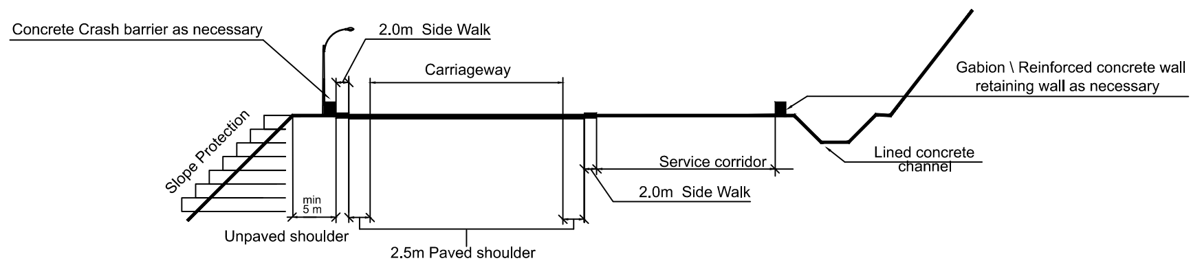
Typical Section :Hill cutting and Embankment on each side
